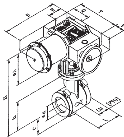
Flangeless valve - Sandwich Actuator RP99-1
