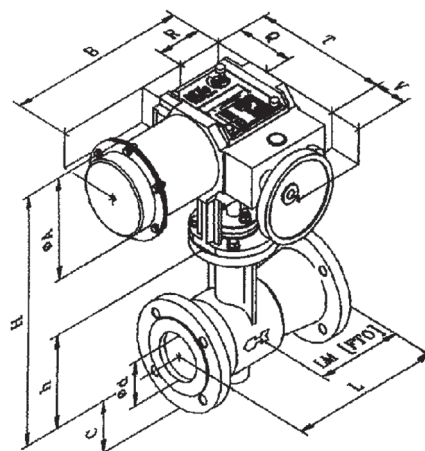
Flanged valve Actuator RP99-1
