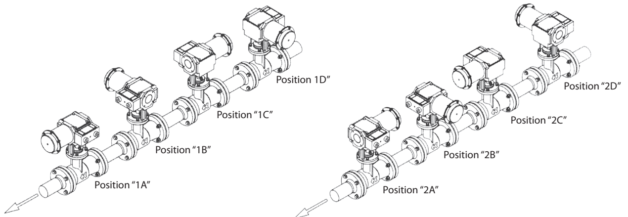
Fig. 5 Possible actuator type RP99 positions to valve axis.
